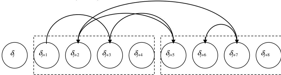
Figure 1: Illustration of the hopping model. The random walk selects successively the variables \delta_{j+1} , \delta_{j+3} , \delta_{j+5} , \delta_{j+2} , \delta_{j+7} , and \delta_{j+6} . The dashed boxes indicated the size (here r = 4 ) of the correlated zones.
