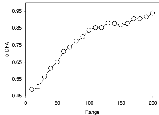
Figure 4: Evolution of the mean \alpha exponent with the length of the Markov chain.
