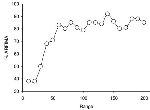
Figure 3: Percentage of series best modeled by ARFIMA models.
