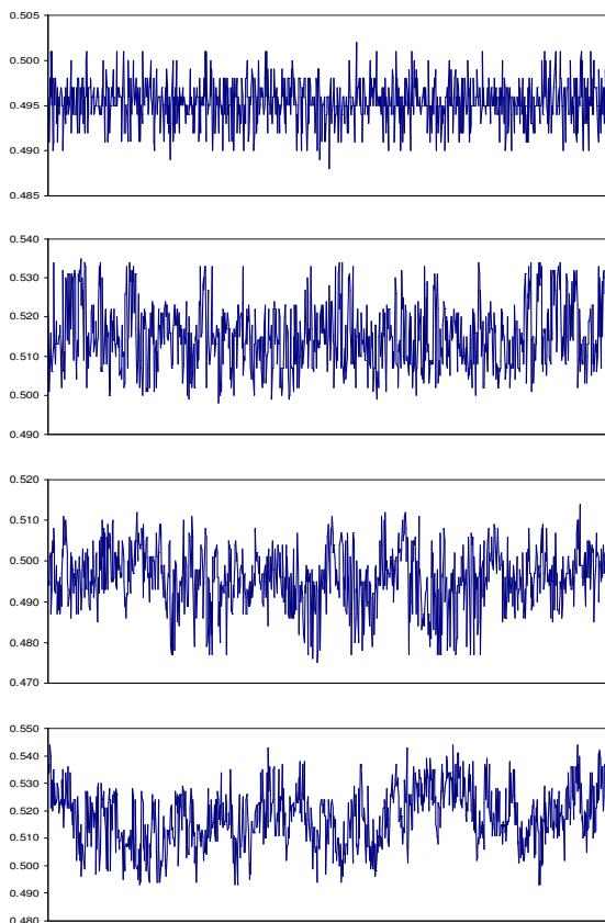
Figure 2: Example series produced by the model. From top to bottom, p = 10 , p = 50 , p = 100 , and p = 200 .
